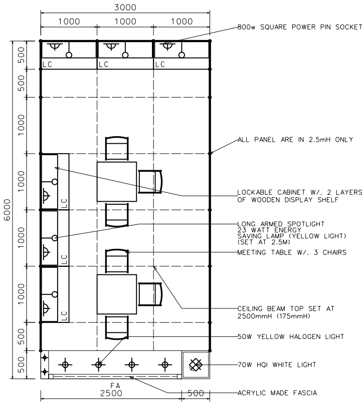
PLAN
