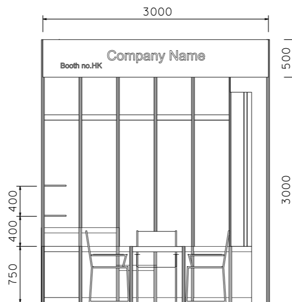
SIDE ELEVATION
