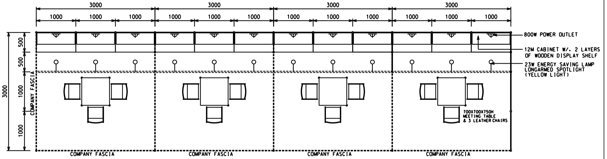
PLAN 12M(W) X 3M(D) X 2.5M(H) LEFT CORNER BOOTH A
