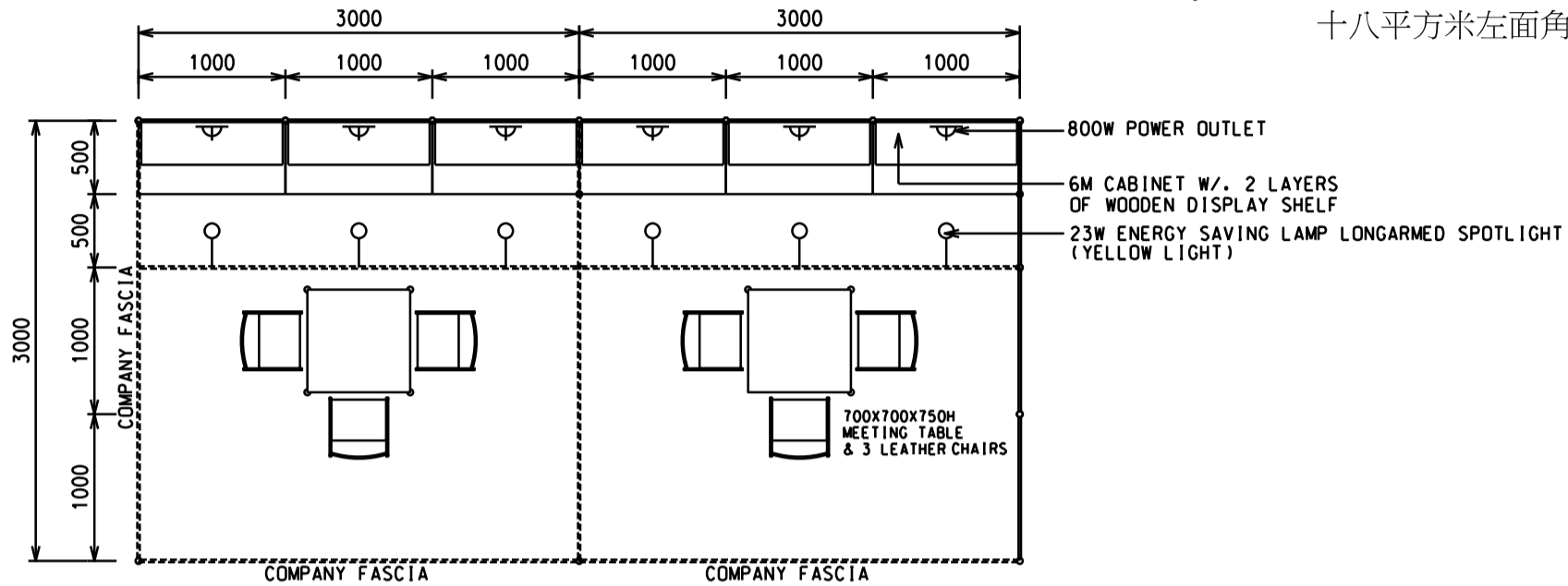
PLAN 6M(W) X 3M(D) X 2.5M(H) LEFT CORNER BOOTH A
