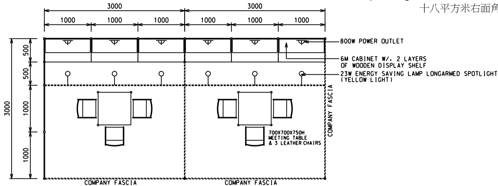
PLAN 6M(W) X 3M(D) X 2.5M(H) RIGHT CORNER BOOTH A
