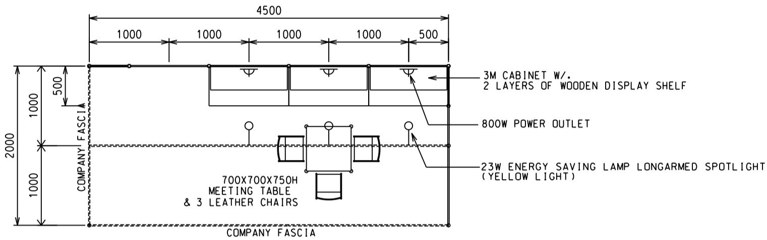
PLAN 4.5M(W) X 2M(D) X 2.5M(H) STANDARD BOOTH A
