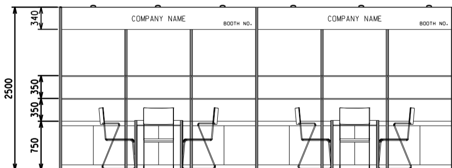
ELEVATION 6M(W) X 6M(D) X 2.5M(H) 3-SIDE OPEN BOOTH A
