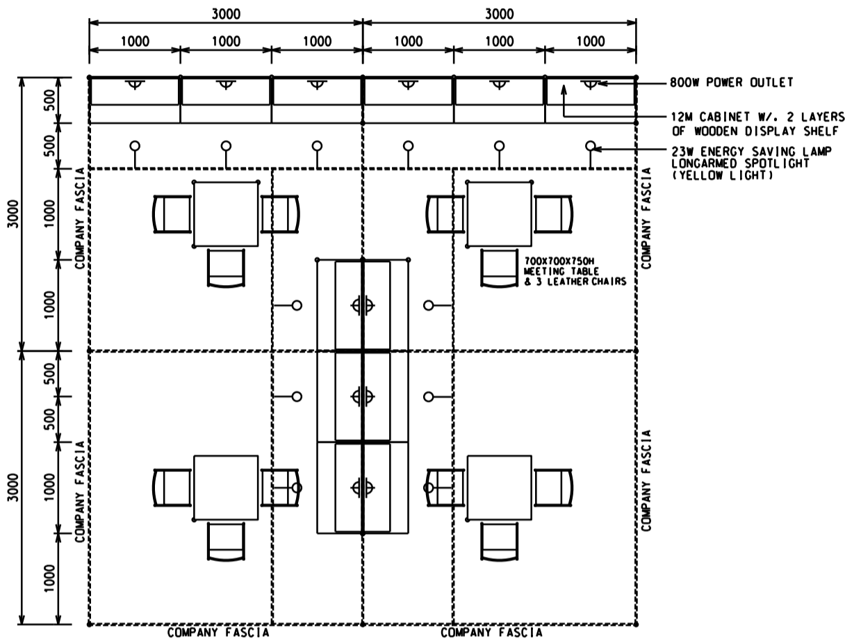
PLAN 6M(W) X 6M(D) X 2.5M(H) 3-SIDE OPEN BOOTH A
