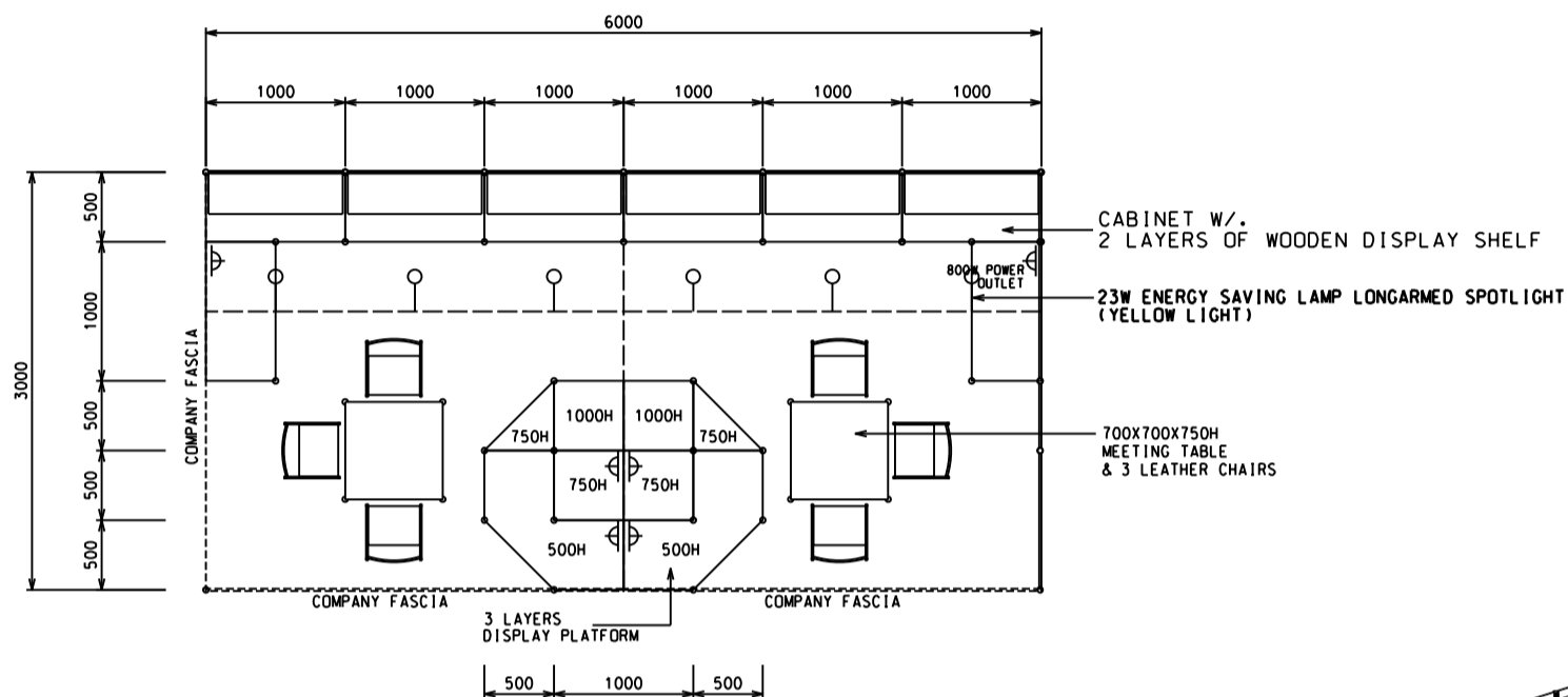
PLAN 6M(W) X 3M(D) X 2.5M(H) LEFT CORNER BOOTH B
