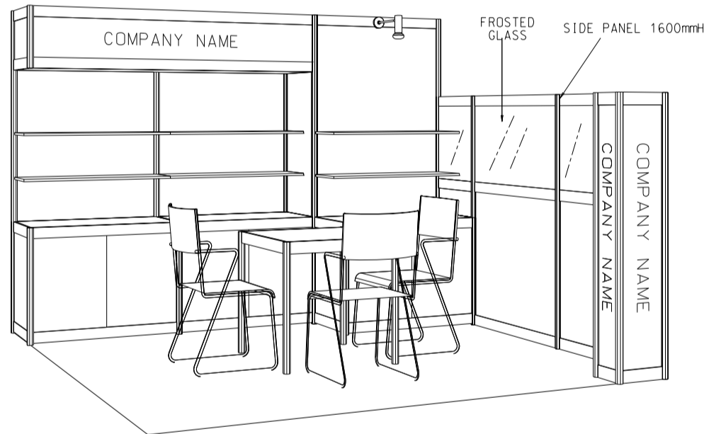
PERSPECTIVE
