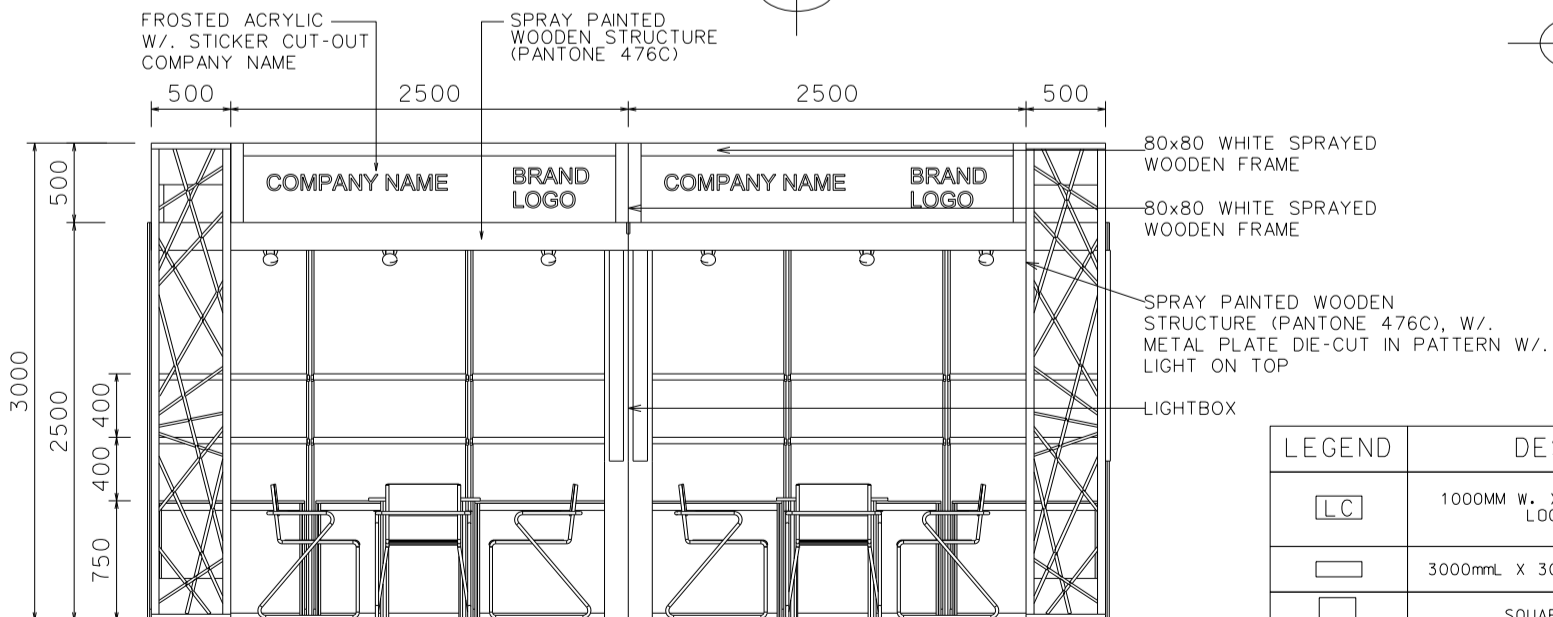
SIDE ELEVATION
