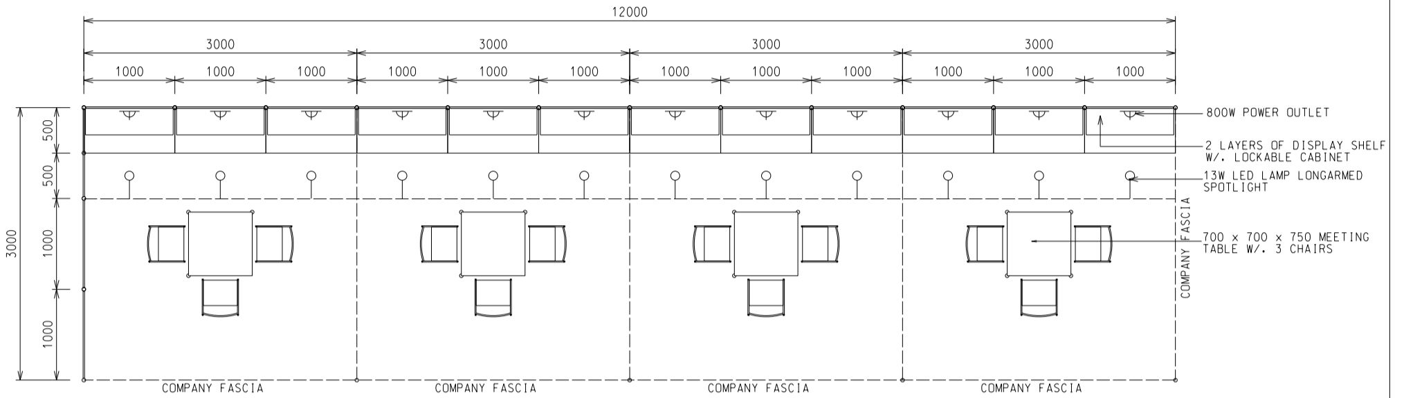
PLAN 12M(W) X 3M(D) X 2.5M(H) Right Corner Booth A
