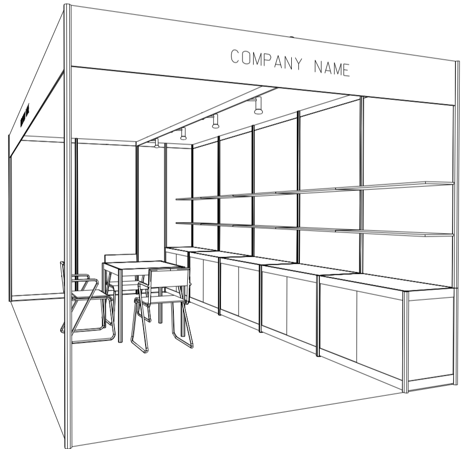
PERSPECTIVE 3M(W) X 5M(D) X 2.5M(H) Left Corner Booth A
