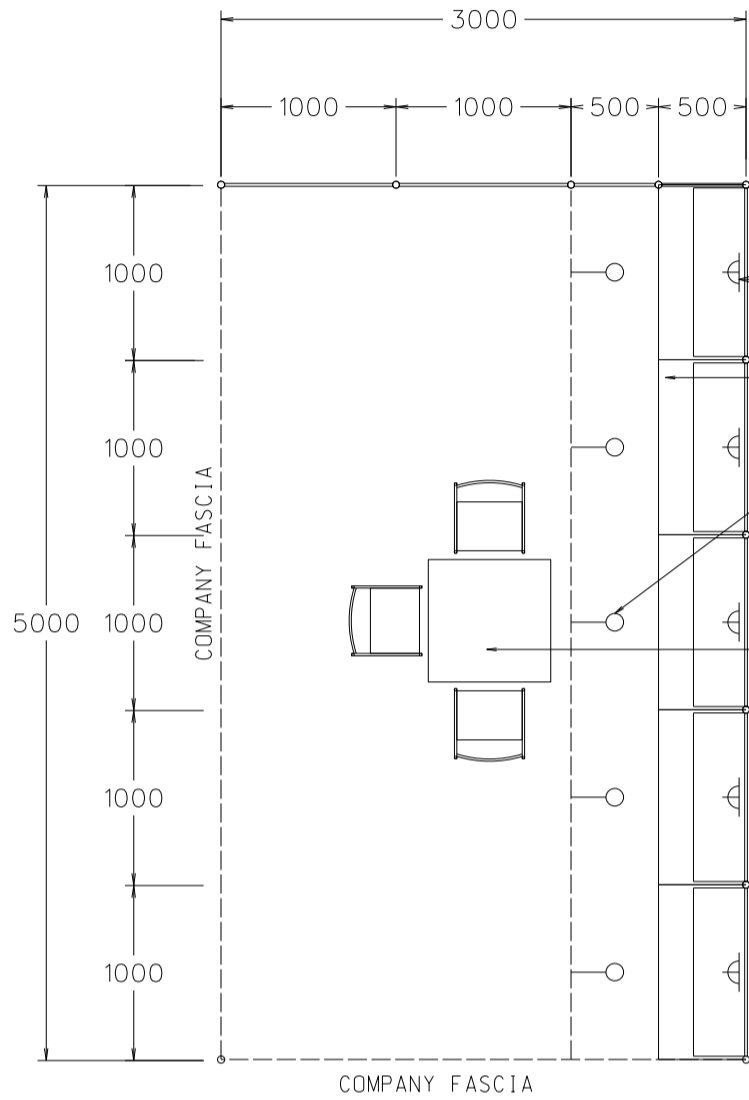
PLAN 3M(W) X 5M(D) X 2.5M(H) Left Corner Booth A
