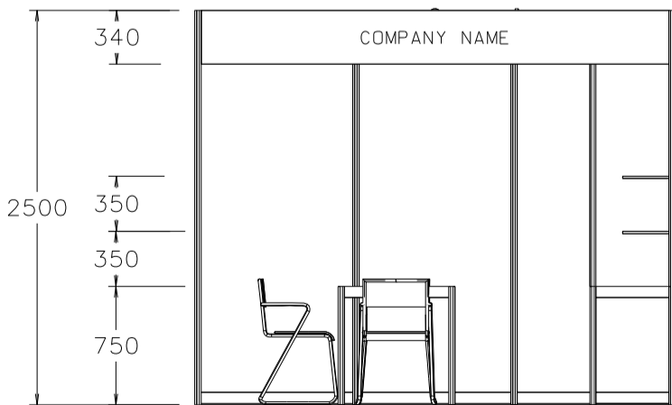
ELEVATION 3M(W) X 5M(D) X 2.5M(H) Left Corner Booth A
