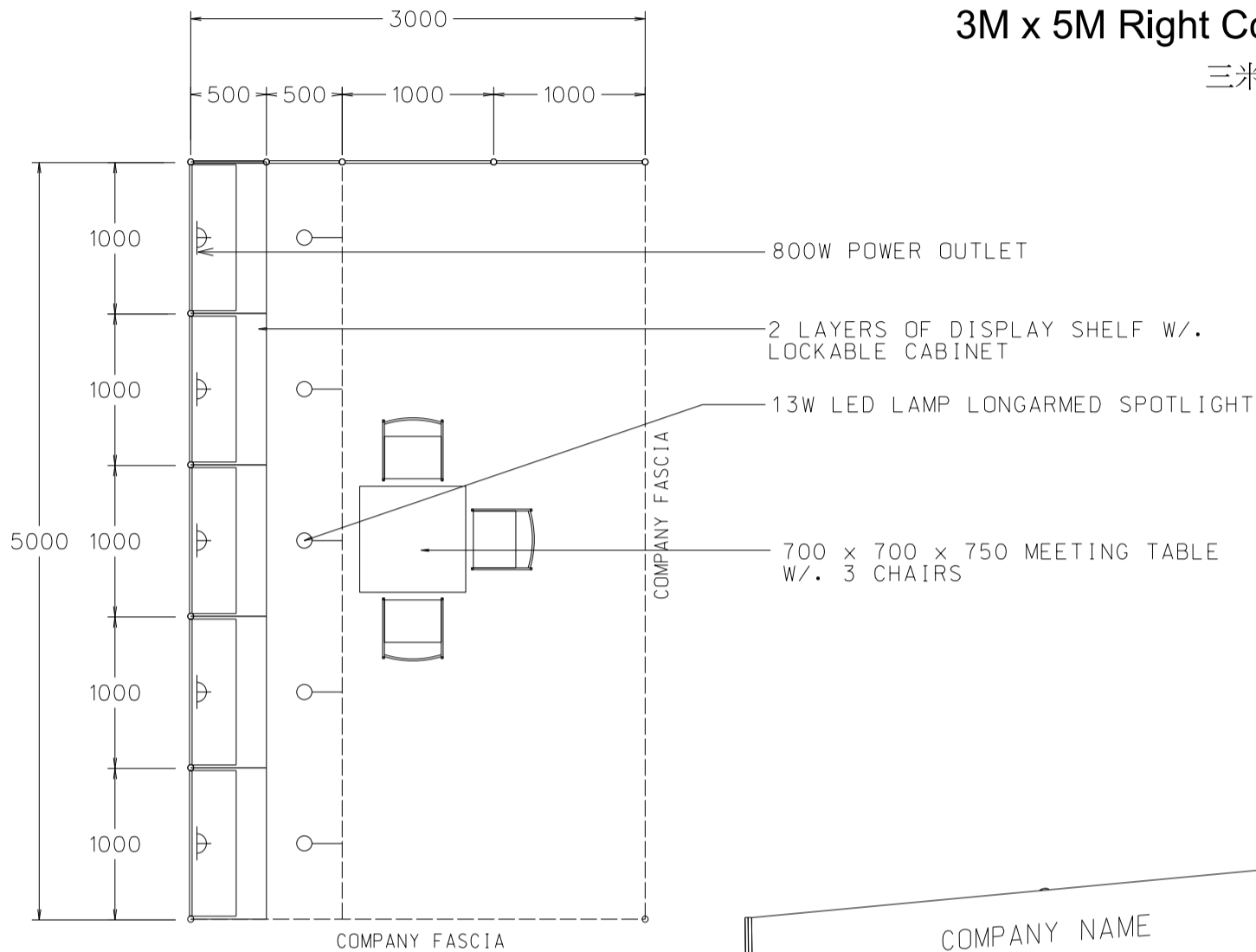
PLAN 3M(W) X 5M(D) X 2.5M(H) Right Corner Booth A
