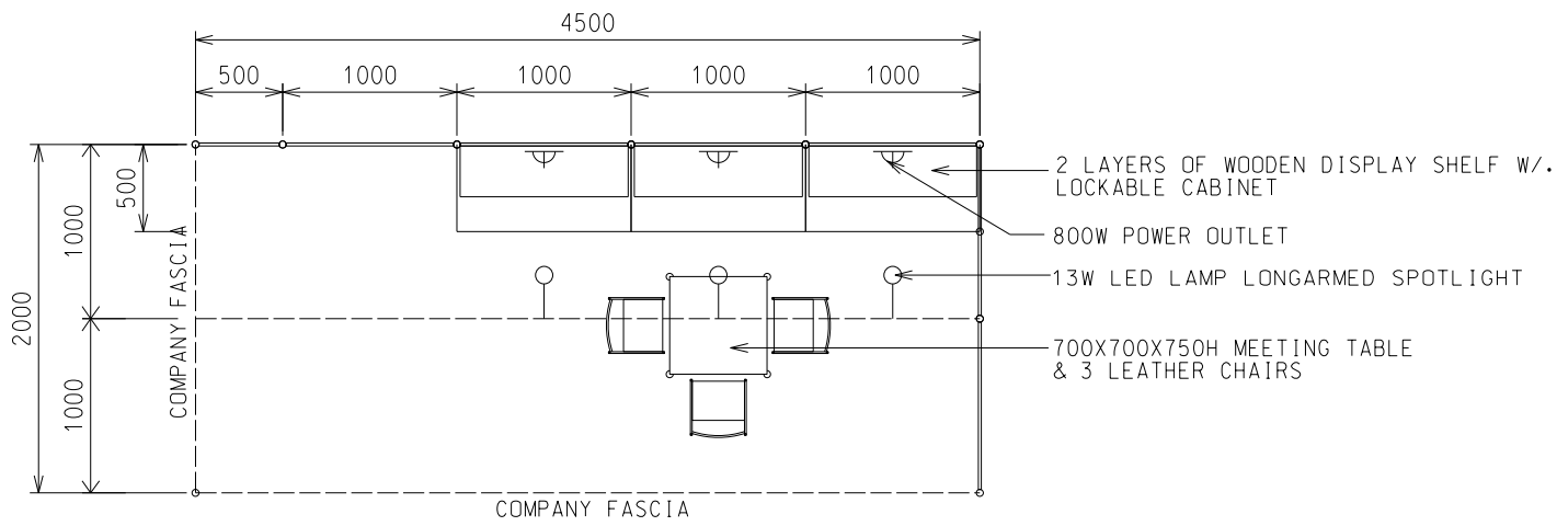
PLAN 4.5M(W) X 2M(D) X 2.5M(H) Left Corner Booth A
