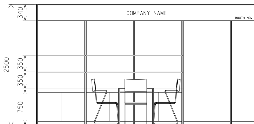
ELEVATION 4.5M(W) X 2M(D) X 2.5M(H) Right Corner Booth A
