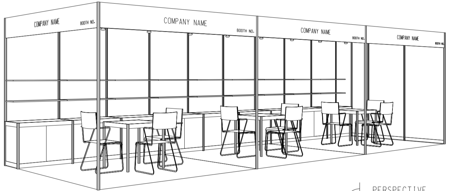
PERSPECTIVE 9M(W) X 3M(D) X 2.5M(H) Left Corner Booth A
