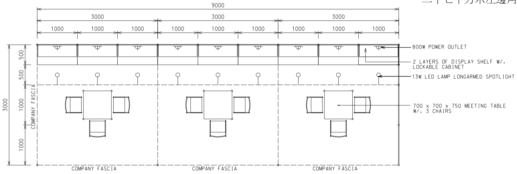
PLAN 9M(W) X 3M(D) X 2.5M(H) Left Corner Booth A
