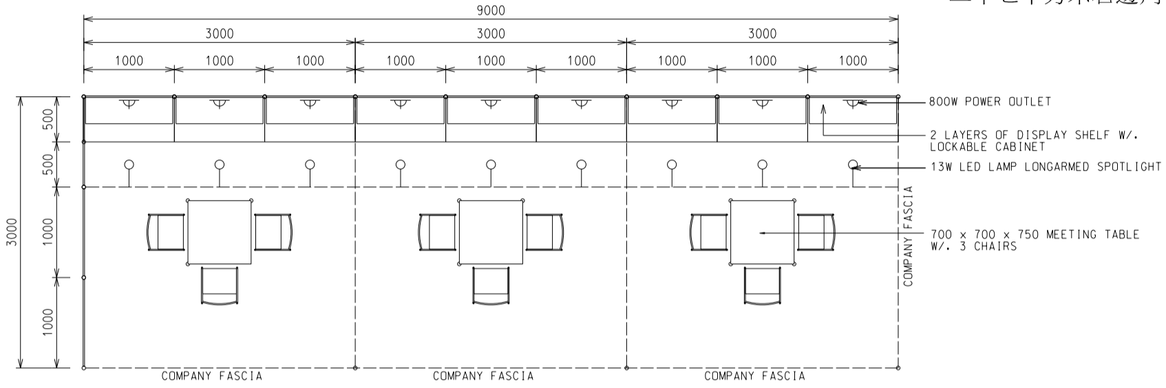
PLAN 9M(W) X 3M(D) X 2.5M(H) Right Corner Booth A
