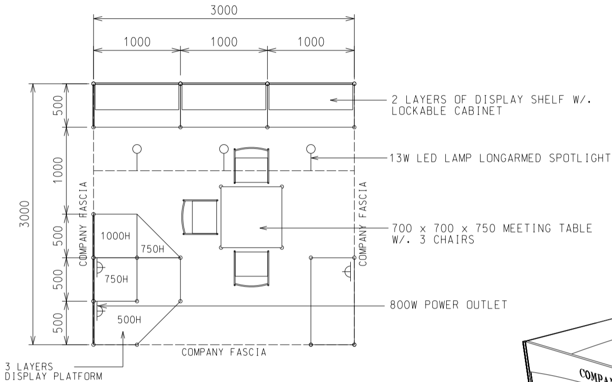
PLAN 3M(W) X 3M(D) X 2.5M(H) Peninsula Booth B
