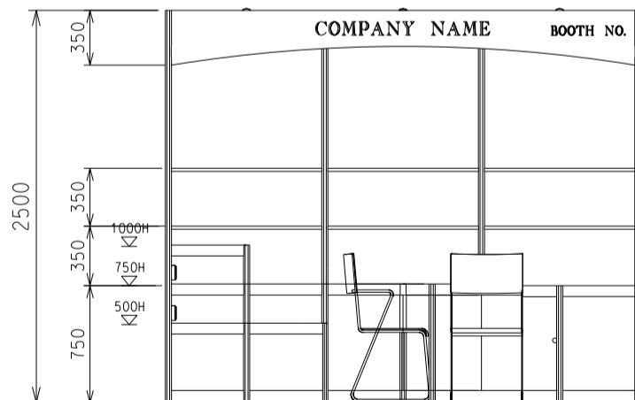
ELEVATION 3M(W) X 3M(D) X 2.5M(H) Peninsula Booth B
