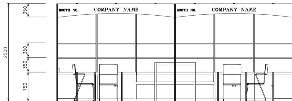
ELEVATION 6M(W) X 3M(D) X 2.5M(H) 3-SIDE OPEN BOOTH B
