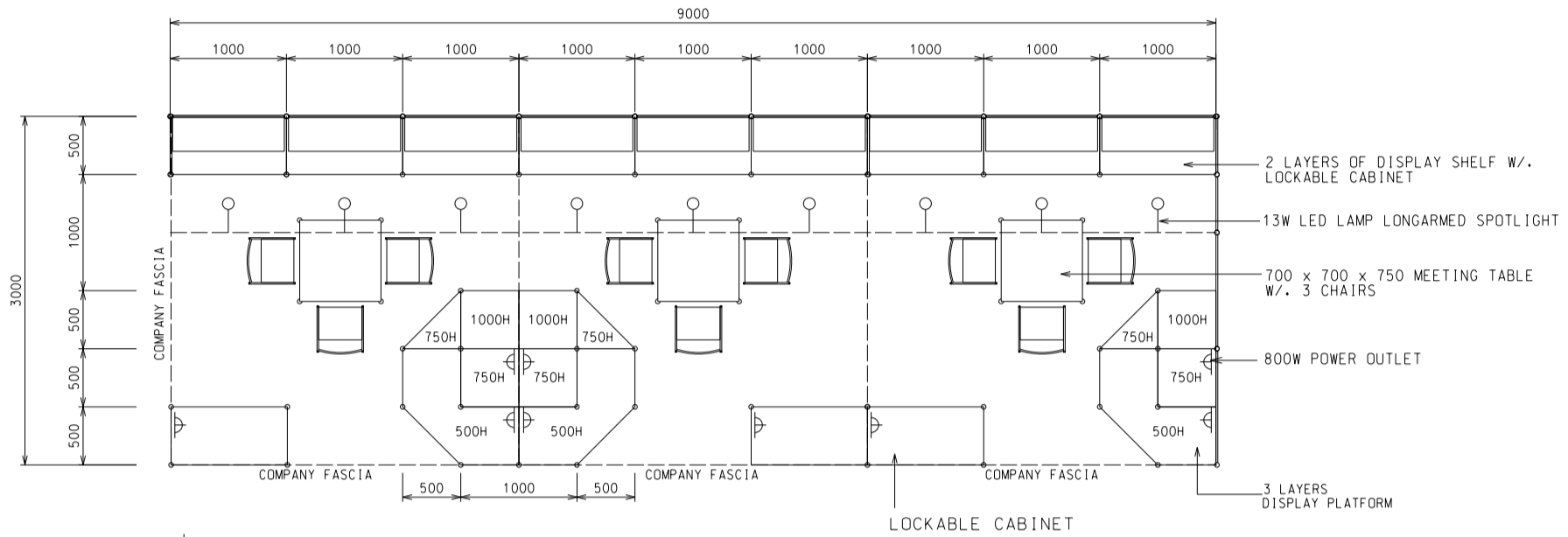
PLAN 9M(W) X 3M(D) X 2.5M(H) LEFT CORNER BOOTH B
