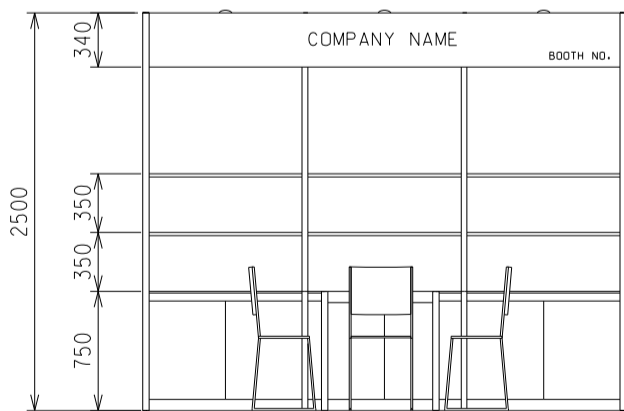
ELEVATION 3M(W) X 3M(D) X 2.5M(H) Peninsula Booth A
