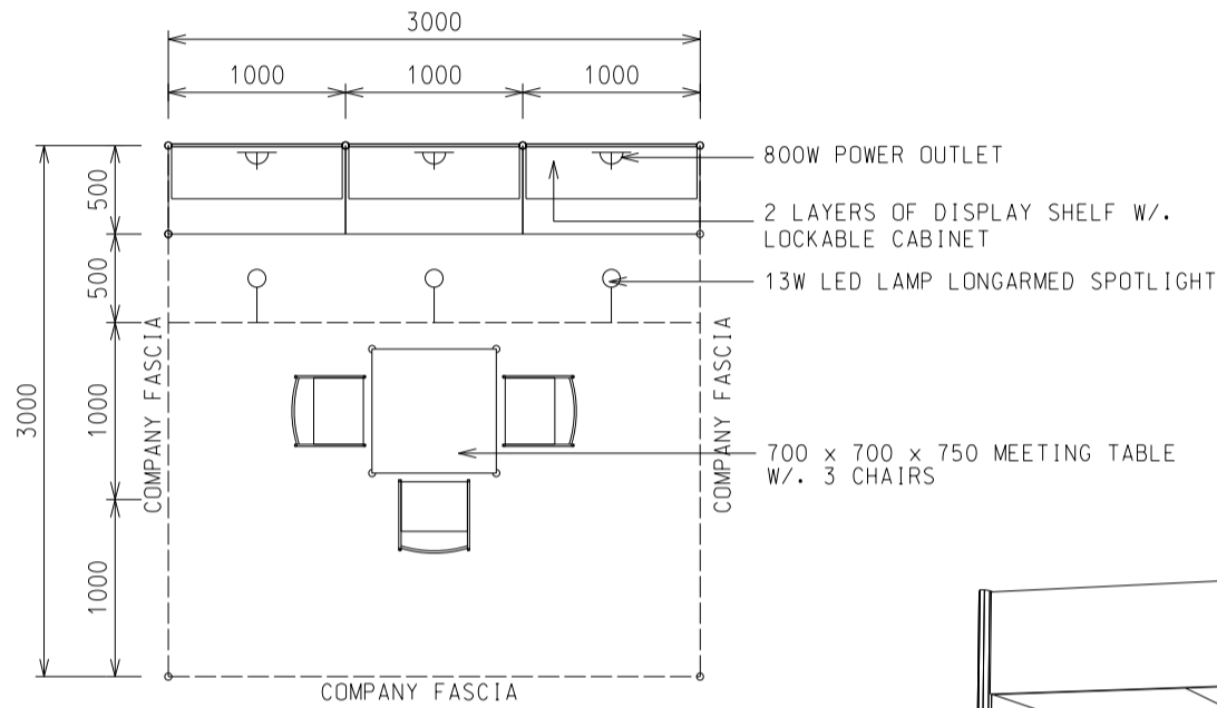
PLAN 3M(W) X 3M(D) X 2.5M(H) Peninsula Booth A
