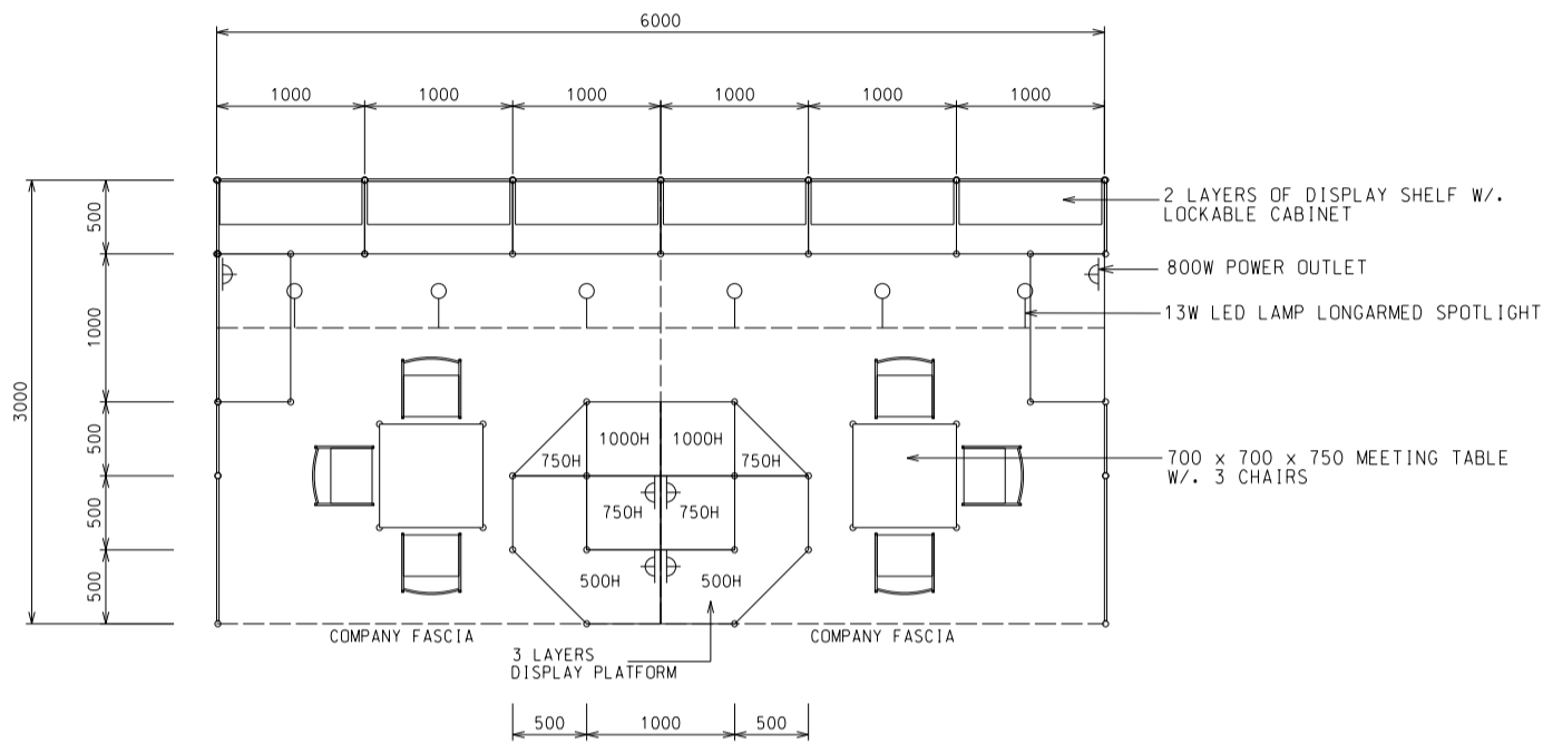
PLAN 6M(W) X 3M(D) X 2.5M(H) STANDARD BOOTH B
