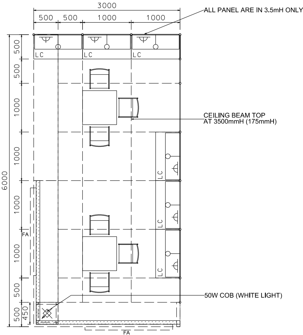
PLAN
